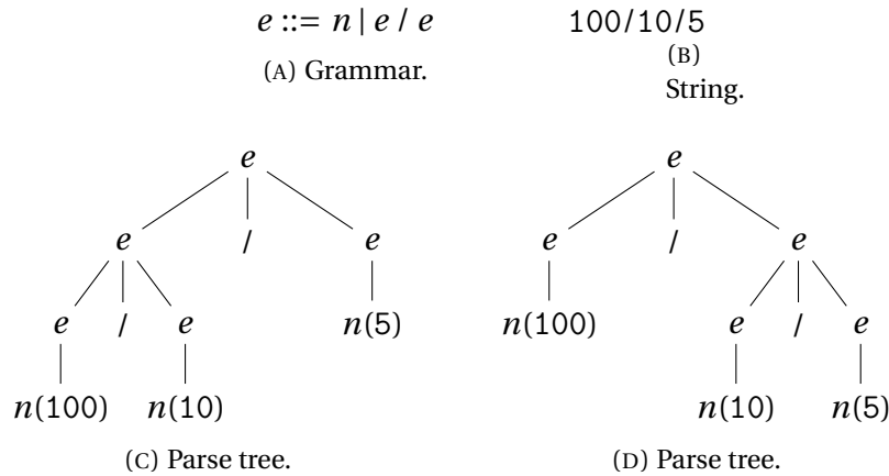
FIGURE 2.1. An ambiguous grammar is exhibited by two parse trees for a string in the language described by the grammar.
